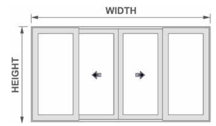
4 pane
