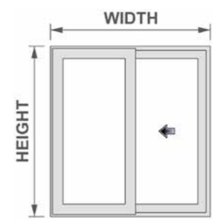
2 pane
